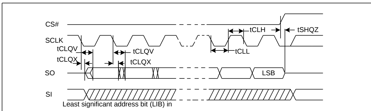
Figure 42. Output Timing
